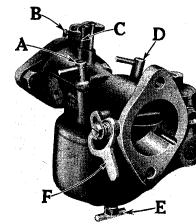
John Deere D carburetor
